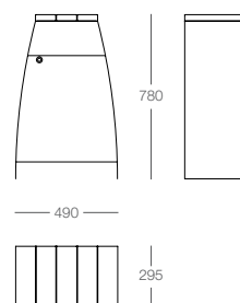
litter bin 35L corbeille 35L papeleira 35L
