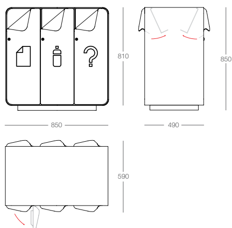
outdoor container 3x50L écopoint outdoor 3x50L ecoponto outdoor 3x50L
