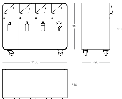
outdoor container 4x50L écopoint outdoor 4x50L ecoponto outdoor 4x50L
