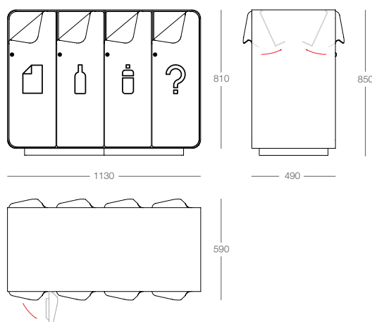
outdoor container 4x50L écopoint outdoor 4x50L ecoponto outdoor 4x50L
