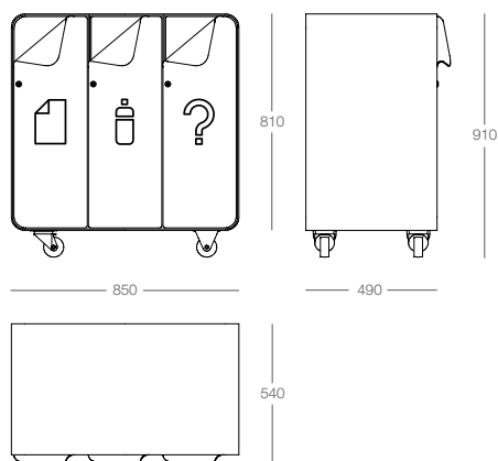
outdoor container 3x50L écopoint outdoor 3x50L ecoponto outdoor 3x50L
