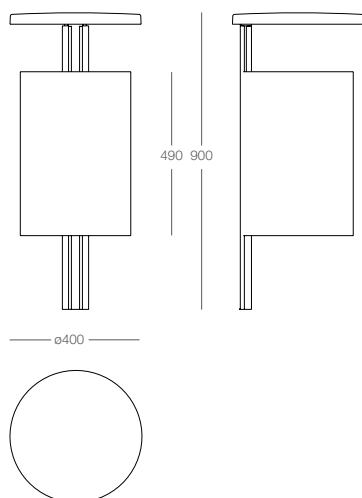
litter bin 40L corbeille 40L papeleira 40L
